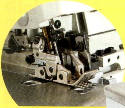
EXTRA HEAVY DUTY TOP FEED MACHINE
